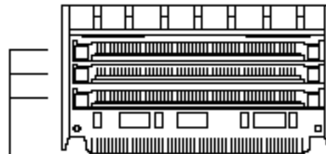
MEMORY EXPANSION BOARD SPARE PN 118739-001
