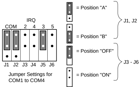
Jumper Block Settings
