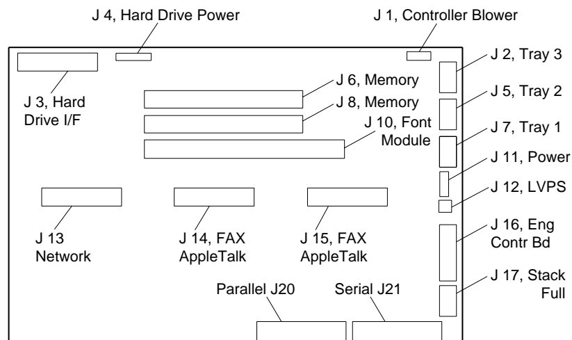
SYSTEM CONTROLLER BOARD
