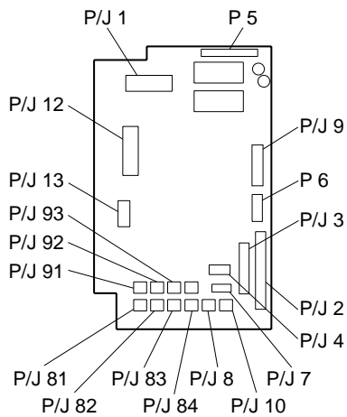
ENGINE CONTROLLER BOARD
