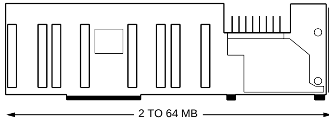
32-BIT 4-SOCKET SYSTEM MEMORY BOARD ASSY NO. 001370
